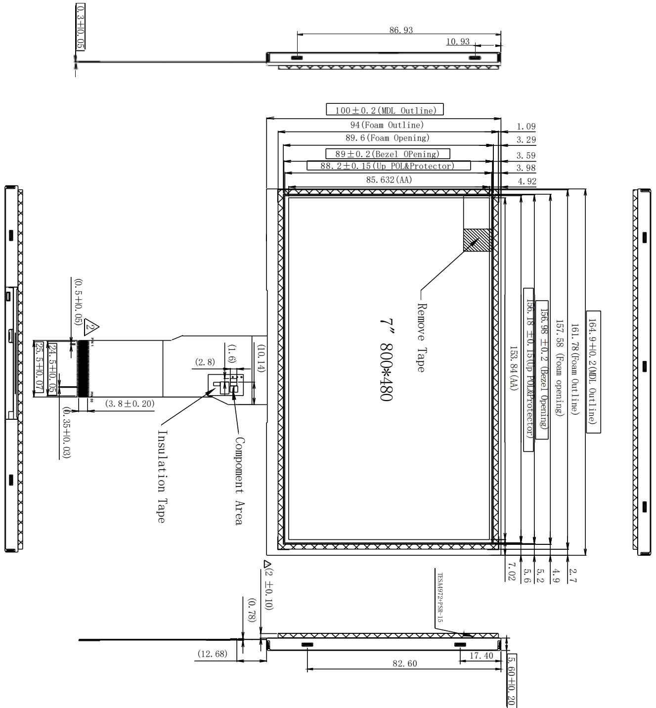
Figure 4. TFT-LCD Module Outline Dimension (Front View)
